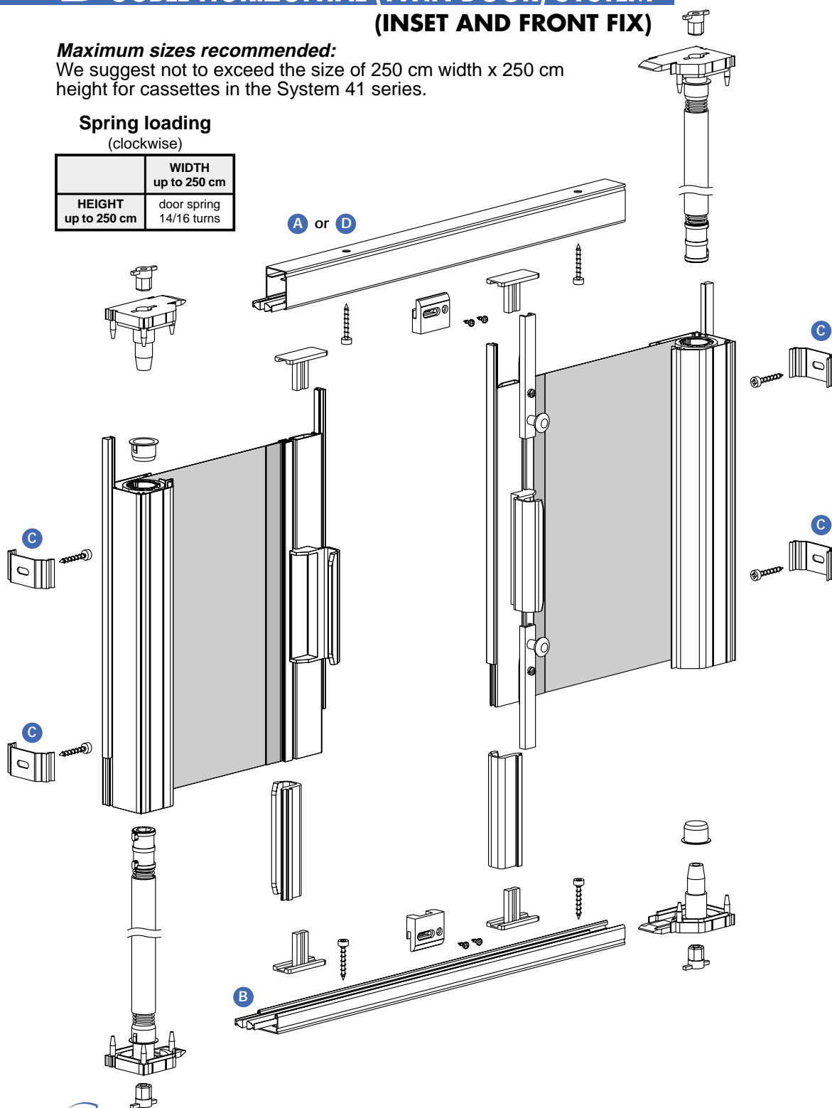
Option for front fix (single & double)
