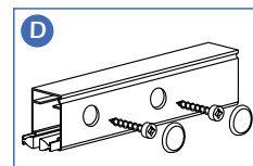
Option for front fix with cap (single & double)
